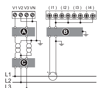
2VT, 1CT ♦
