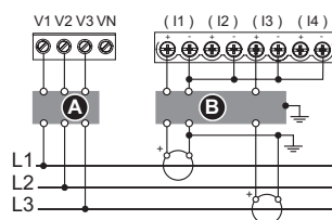
2CT
