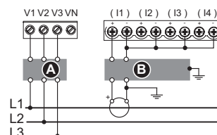
1CT ♦
