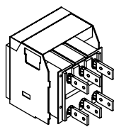
P-Frame Drawout Cradle Connections
