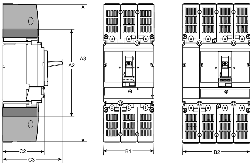
A2: Short A3: Long PV T-Frame Circuit Breaker
