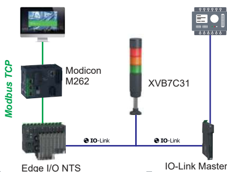
Connectivity with IO-Link protocol
