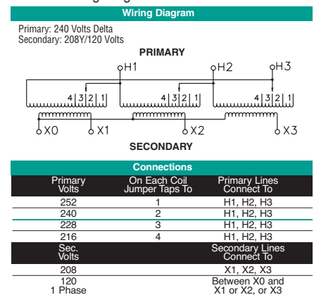
T240F Wiring Diagram & Connections*
