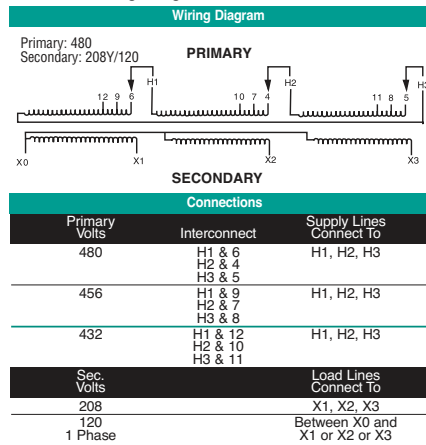
T480D Wiring Diagram & Connections*
