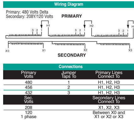
T480A Wiring Diagram & Connections*
