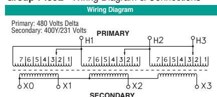
Group T480L Wiring Diagram & Connections*
