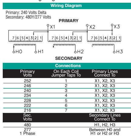
T240D Wiring Diagram & Connections*
