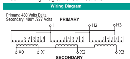
T480P Wiring Diagram & Connections*
