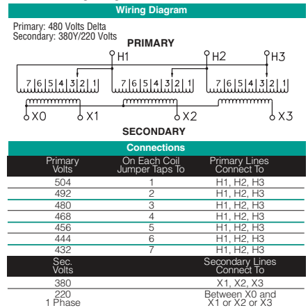
T480I Wiring Diagram & Connections*
