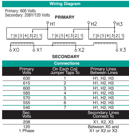
T600B Wiring Diagram & Connections*
