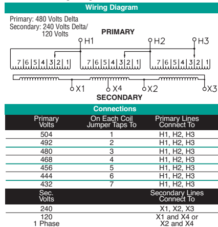
T480G Wiring Diagram & Connections*
