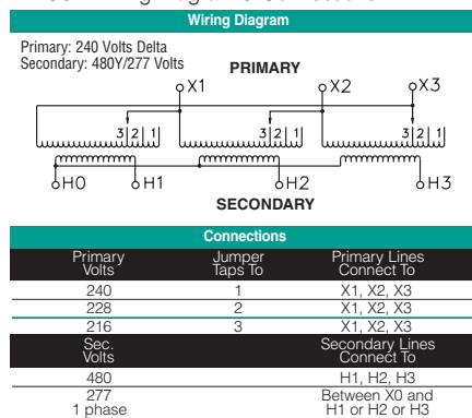
T240G Wiring Diagram & Connections*
