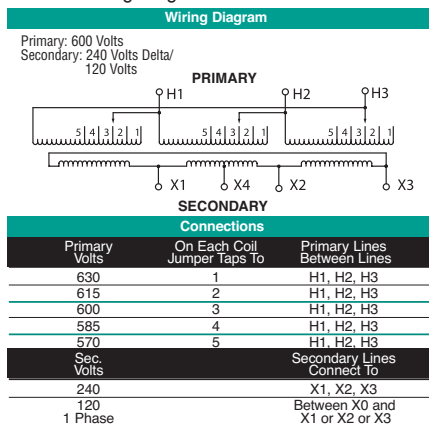
T600F Wiring Diagram & Connections*
