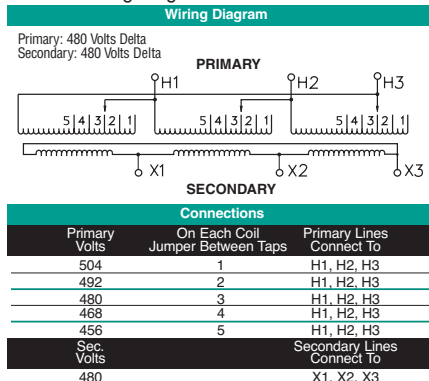
T480F Wiring Diagram & Connections
