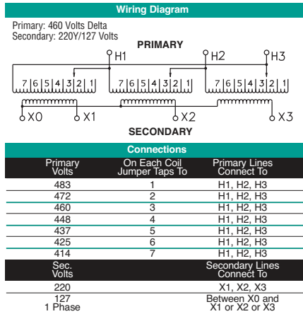
T460A Wiring Diagram & Connections*
