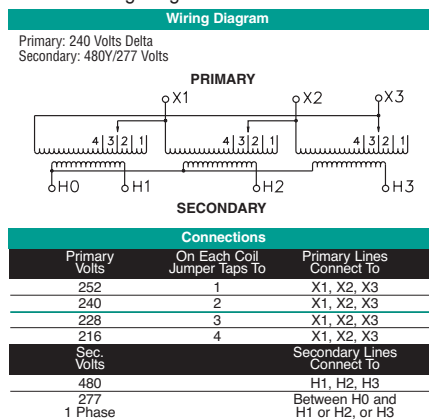
T240E Wiring Diagram & Connections*
