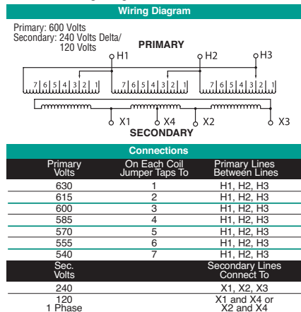
T600D Wiring Diagram & Connections*
