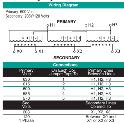
T600G Wiring Diagram & Connections*
