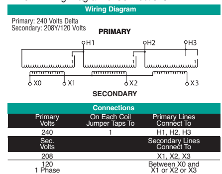
T240I Wiring Diagram & Connections*
