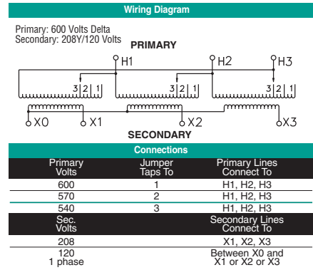
T600A Wiring Diagram & Connections*
