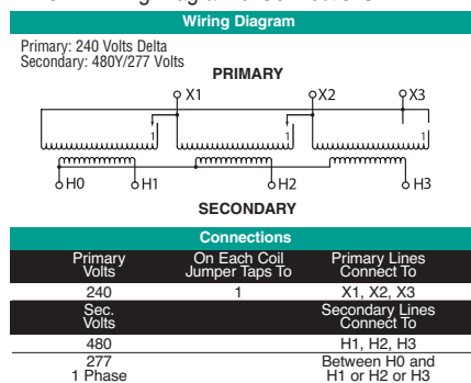
T240H Wiring Diagram & Connections*
