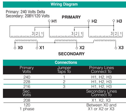
T240A Wiring Diagram & Connections*
