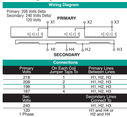
T208L Wiring Diagram & Connections*
