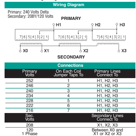
T240B Wiring Diagram & Connections*
