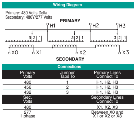
T480C Wiring Diagram & Connections*
