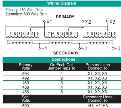
T480V Wiring Diagram & Connections*
