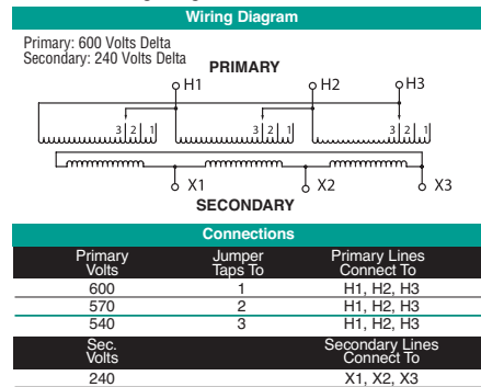
T600E Wiring Diagram & Connections*
