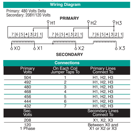
T480E Wiring Diagram & Connections*
