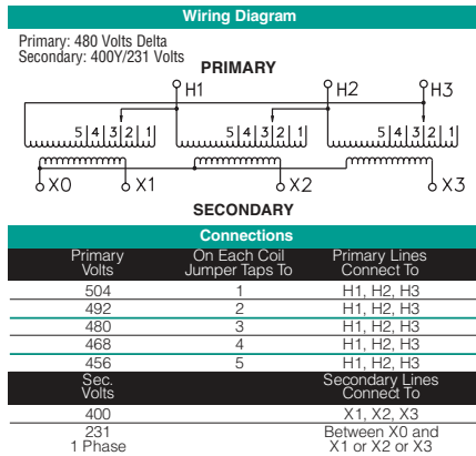
T480U Wiring Diagram & Connections*
