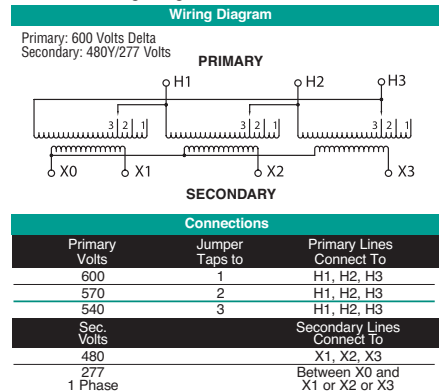
T600H Wiring Diagram & Connections*
