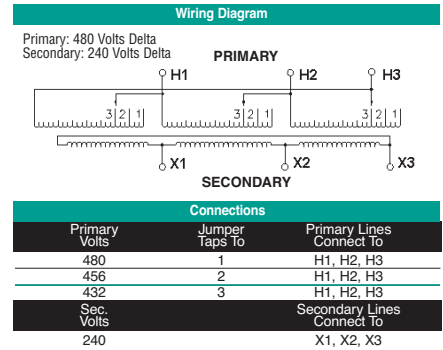
T480B Wiring Diagram & Connections*
