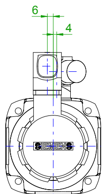
back view
