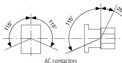
AC contactors
