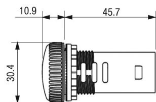
Pilot Light Devices (D7D-P)
