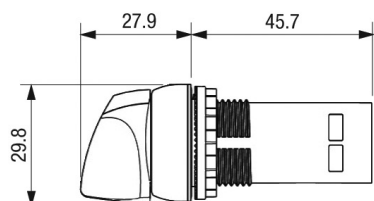
Momentary Pushbutton Device - Extended (D7D-E)
