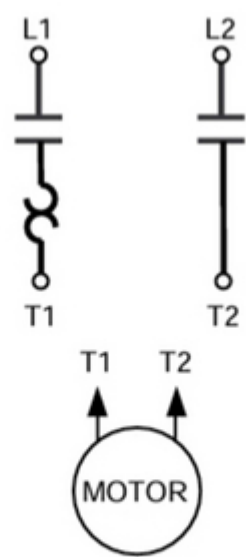
2-Pole, 1-Phase
