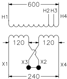
SERIES CONNECTION
