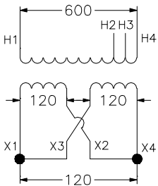
PARALLEL CONNECTION
