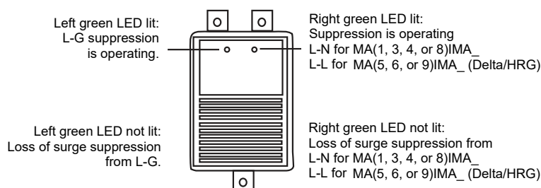
Figure 9: MA Module LEDs
