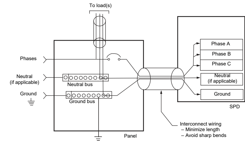
Figure 2: Surge Protective Device Wiring Practice
