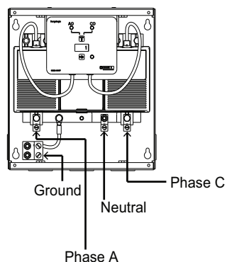
Figure 4: Single-Phase, Three-Wire Grounded Installation
