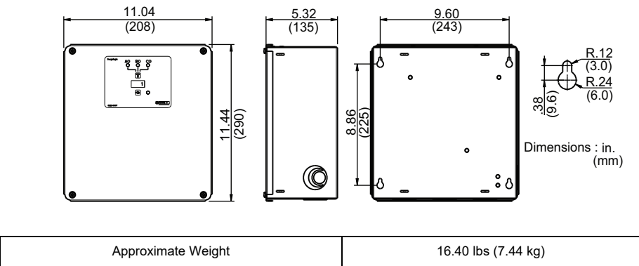
Figure 3: 11 x 12 in. NEMA 1 Enclosures
