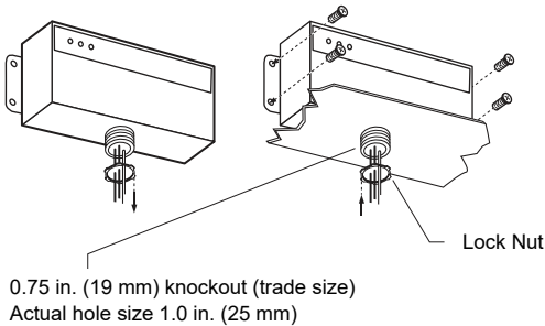
Figure 4 – Mounting unit
