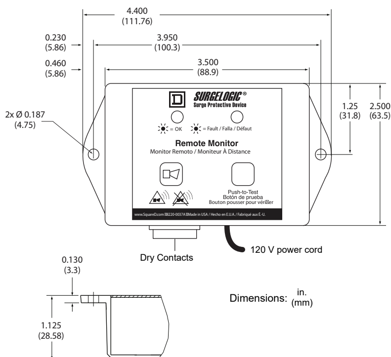
Figure 10: Remote Monitor Option (TVS12RMU)
