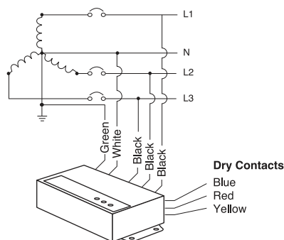
Figure 7: Three-Phase, three- or four-Wire, High-Leg Delta Installation
