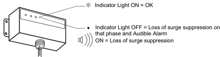
Figure 9: Diagnostic Operation
