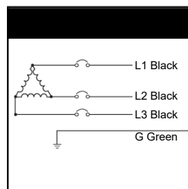
Figure 10: Three-Phase, Three-Wire, Delta Installation
