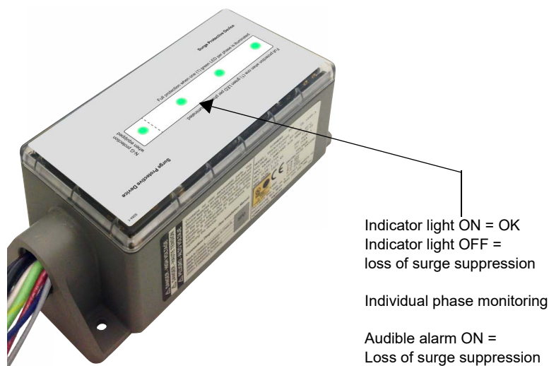
Figure 12: Diagnostic Operation
