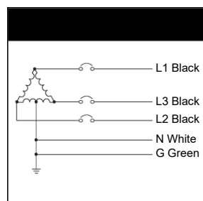
Figure 9: Three-Phase, three- or four-Wire, High-Leg Delta Installation 2
