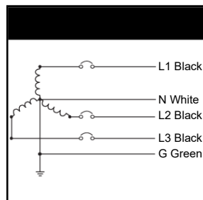
Figure 8: Three-Phase, three- or four-Wire, Grounded WYE Installation 1
