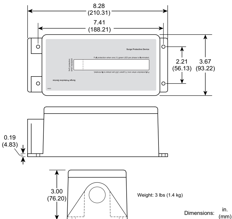
Figure 11: General Dimensions
