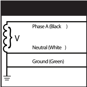
Figure 7: Single-Phase, Two-Wire, Ground
