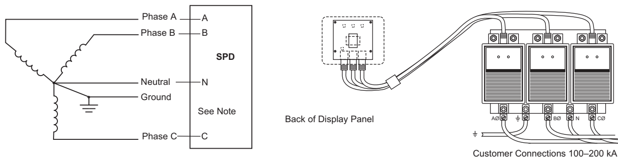
Figure 5 – Three-Phase, Three- or Four-Wire, Grounded Wye Installation
