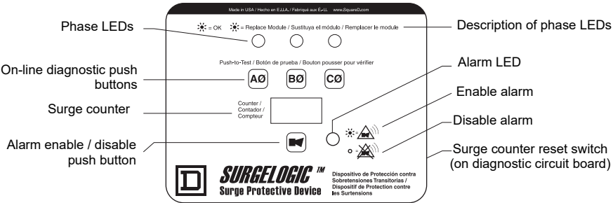
Figure 10 – Three-Phase Diagnostic Display Panel with Surge Counter
