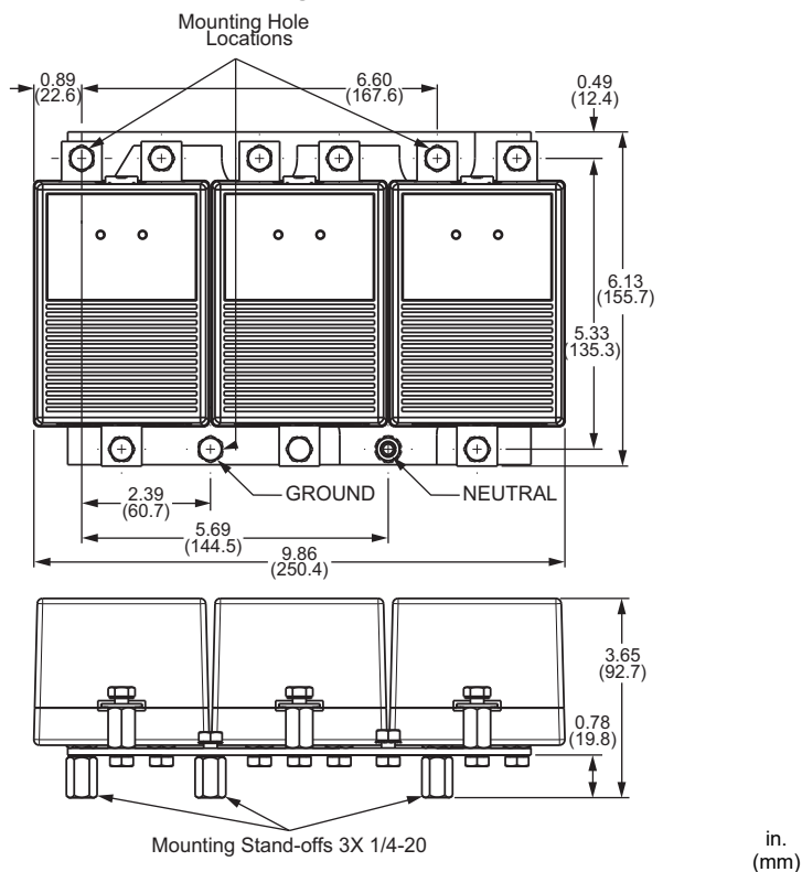
Figure 3 – Dimensions and Mounting
