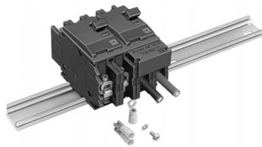
2P DIN-Mounted QOU Circuit Breaker
