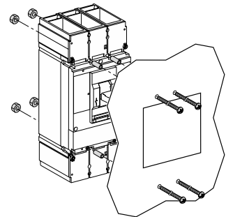
Flush Mounting
