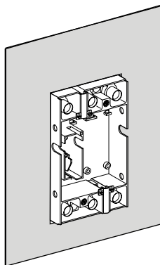
Mounting Through a Panel
