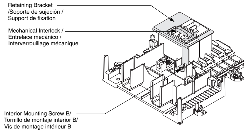
Figure / Figura / Figure 3 : Mechanical Interlock and Retaining Bracket Secured to Base / Entrelace mecánico y soporte de sujeción sujetos a la base / Interverrouillage mécanique et
