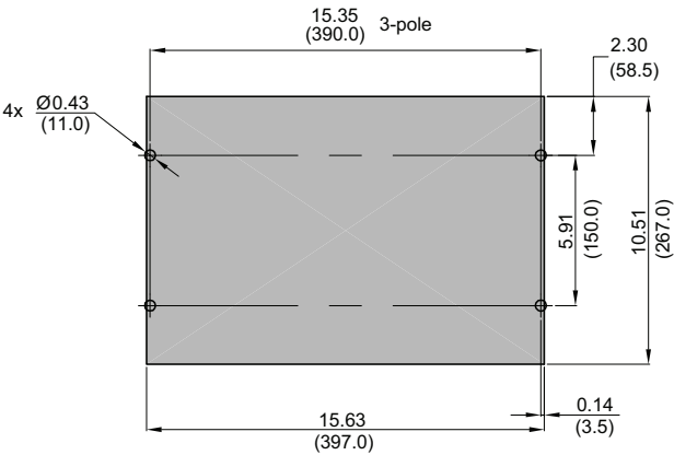
Accessory Cover Escutcheon Cutout
