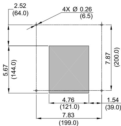
Handle Escutcheon Cutout (Toggle Mech Only)
