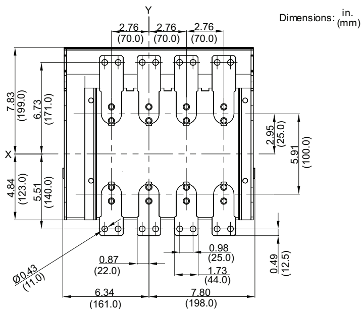
Back View
