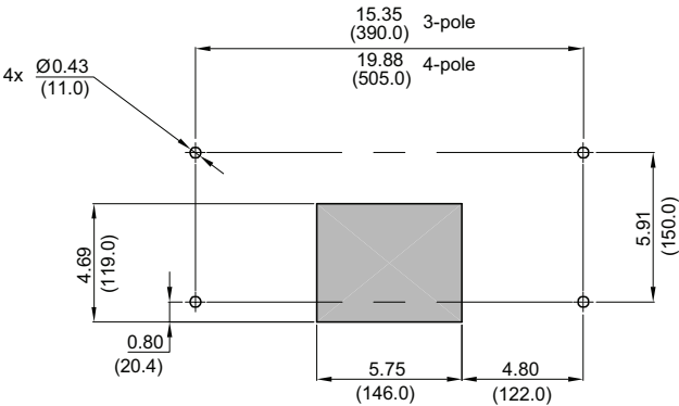
Handle Cutout
