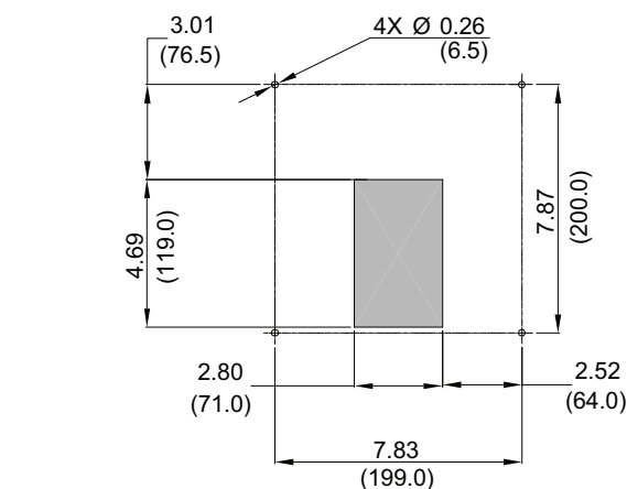
Handle Cutout (Toggle Mech Only)
