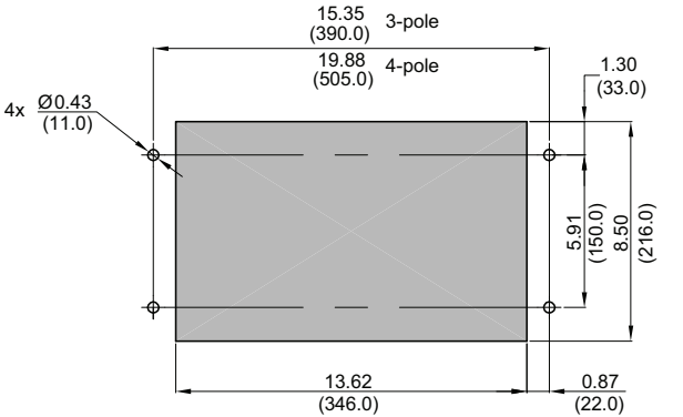
Accessory Cover Cutout
