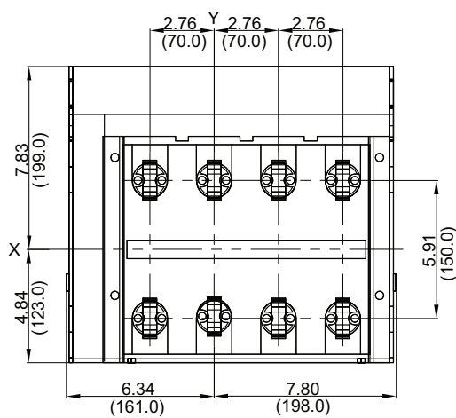
Back View
