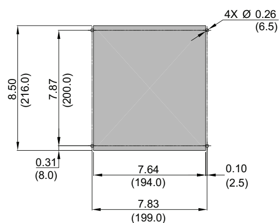
Accessory Cover Cutout
