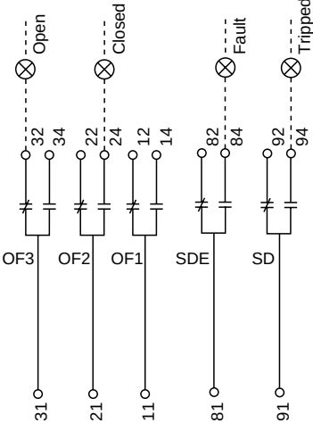
Alarm Contact
