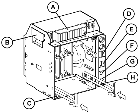
Cradle
