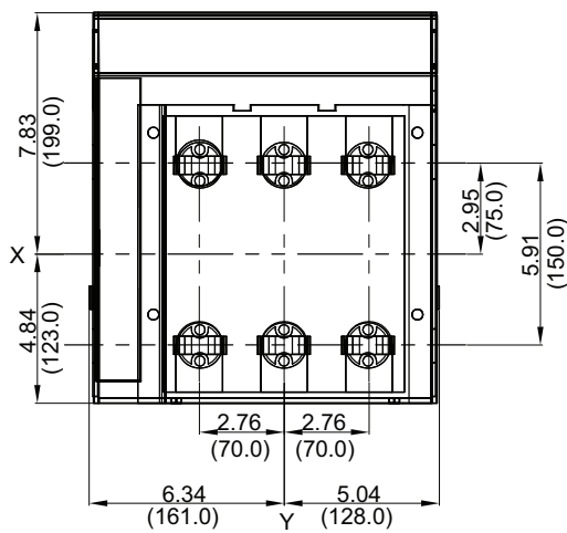
Back View
