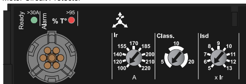
MicroLogic 2.2M and 2.3M Trip Units Ii=4800A
