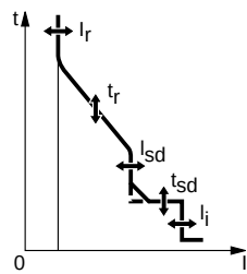
MicroLogic 5.0 Basic Trip Unit Settings
