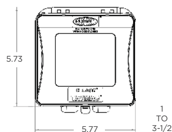
MR420
