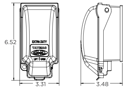
MX3200
