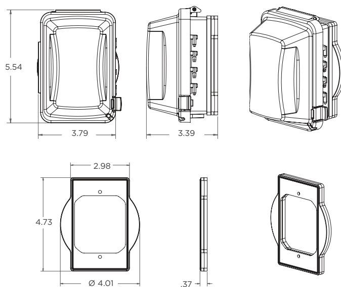
MM710
