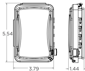
MM110
