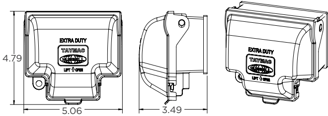
MX3300
