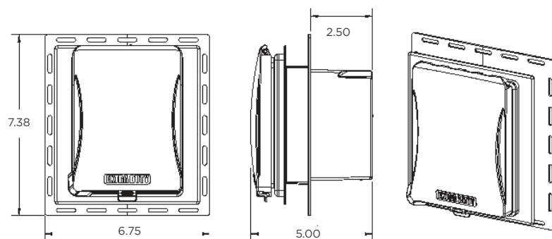
MR420
