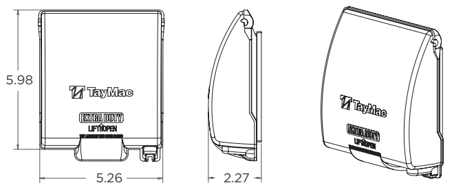
MX7280S
