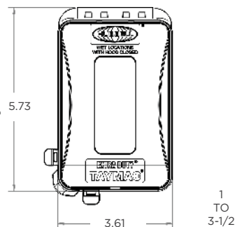
ML500
