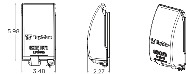
MX4280S
