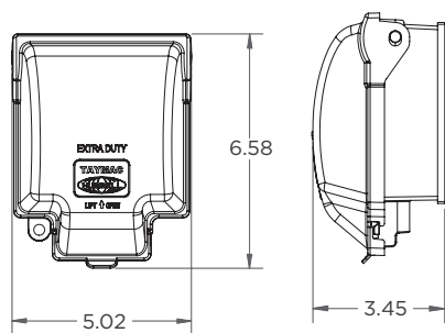
MX6200
