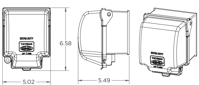
MX7200
