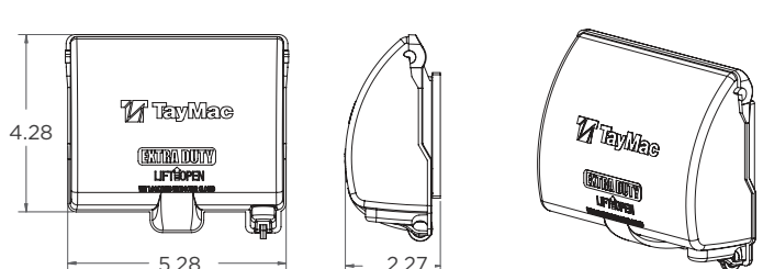
MX4380S
