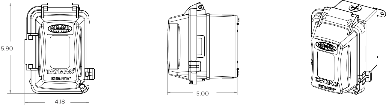
MKG420CS
