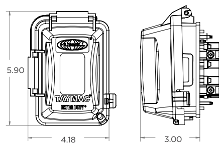
MM420
