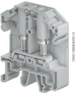
RGW6
