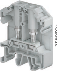
RGW25-M5
