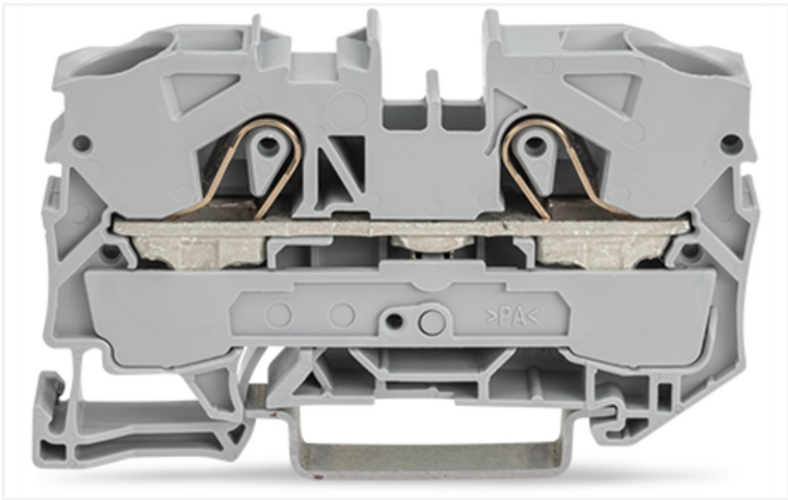
Through terminal block, 2010 Series, Push-in CAGE CLAMP®
