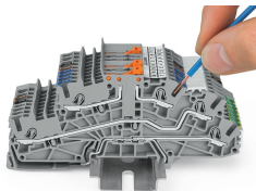
Inserting a conductor via push-in termination. Solid conductors with cross-sections from either one size above, or up to two sizes below, the rated cross-section can be simply pushed in – no tools needed.
