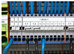
Adjacent Jumpers for Continuous Commoning (Item No. 2002-400)
