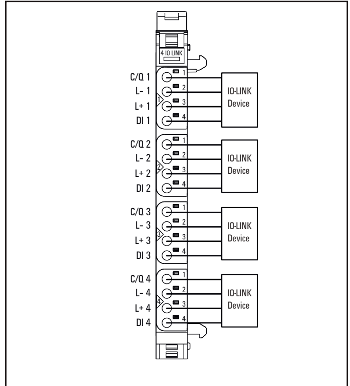
Connection diagram UR20-4COM-IO-LINK-V2
