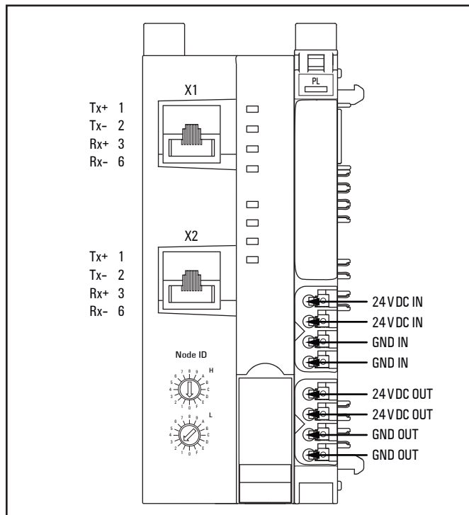
Connection diagram UR20-FBC-PL
