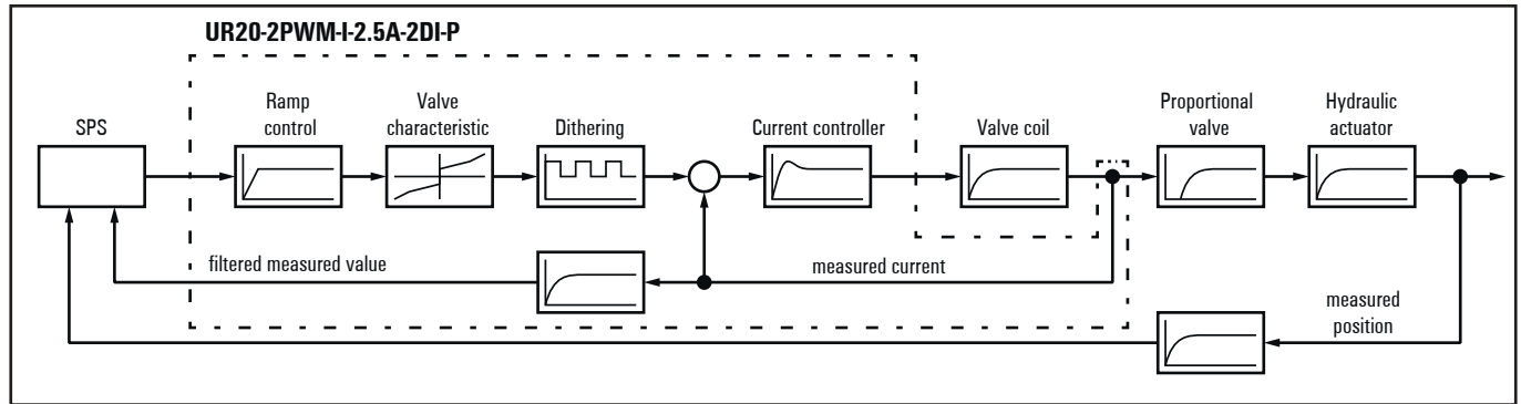
Example: current-controlled PWM module in cascade control for positioning a hydraulic actuator
