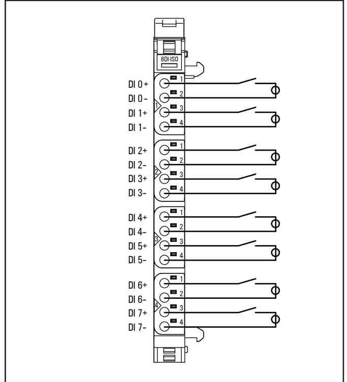
Connection diagram UR20-8DI-ISO-2W
