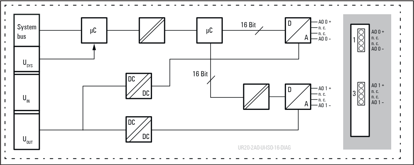
Block diagram UR20-2AO-UH-S0-16-DIAG
