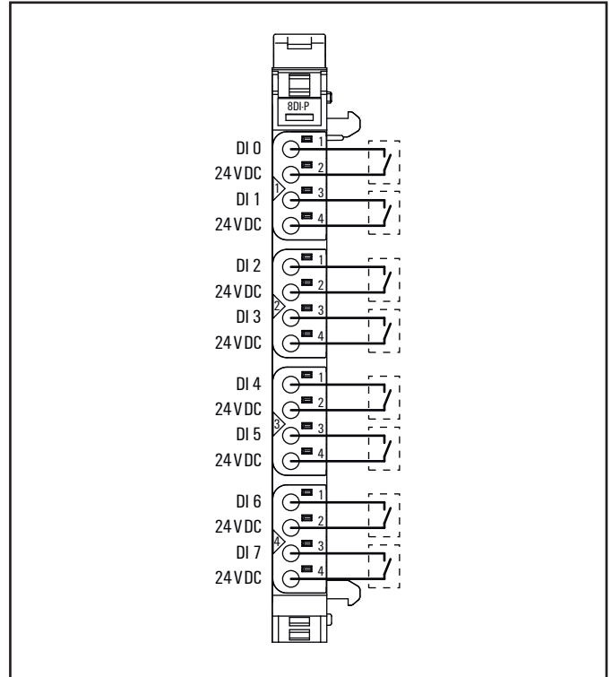
Connection diagram UR20-8DI-P-2W
