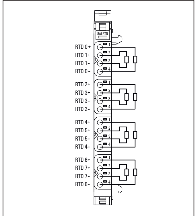
Connection diagram UR20-8AI-RTD-DIAG-2W
