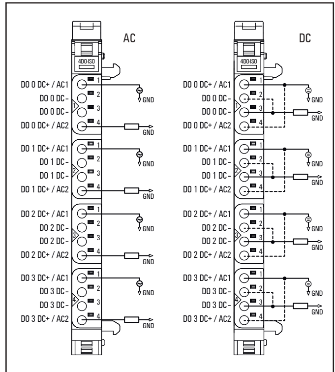
Connection diagram UR20-4DO-ISO-4A
