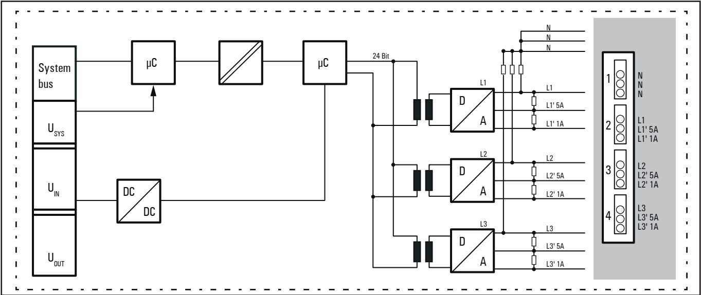
Block diagram UR20-3EM-230V-AC
