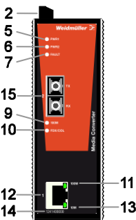
Front Panel View IE-MC-VL-1TX-1SC/1SCS
