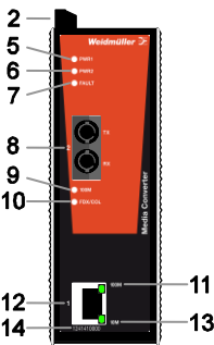
Front Panel View IE-MC-VL-1TX-1ST
