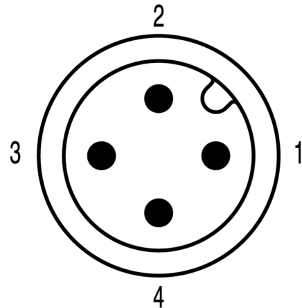
Pole scheme
