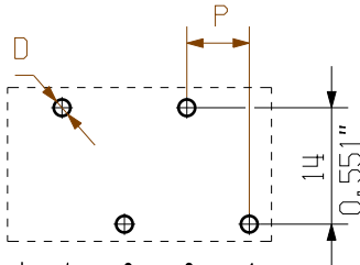
Hole pattern
