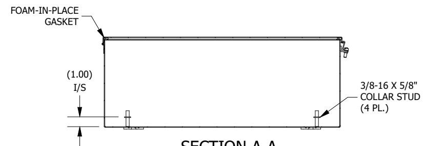
SECTION A-A (INSIDE BOTTOM OF ENCLOSURE)
