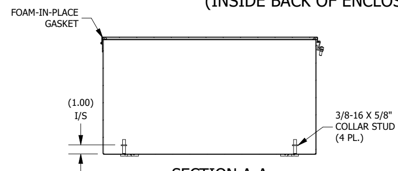
SECTION A-A (INSIDE BOTTOM OF ENCLOSURE)
