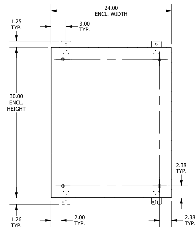
SECTION C-C (INSIDE BACK OF ENCLOSURE)
