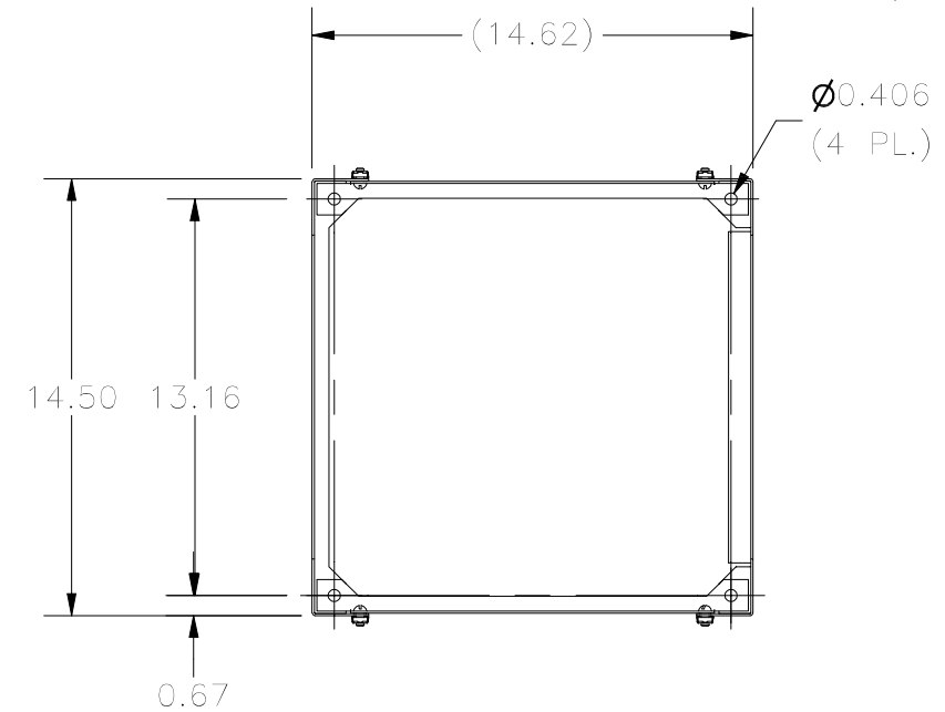
FRONT VIEW (SWING PANEL REMOVED)
