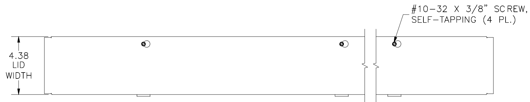
TOP VIEW
