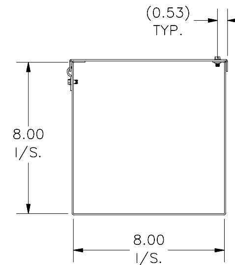
RIGHT VIEW
