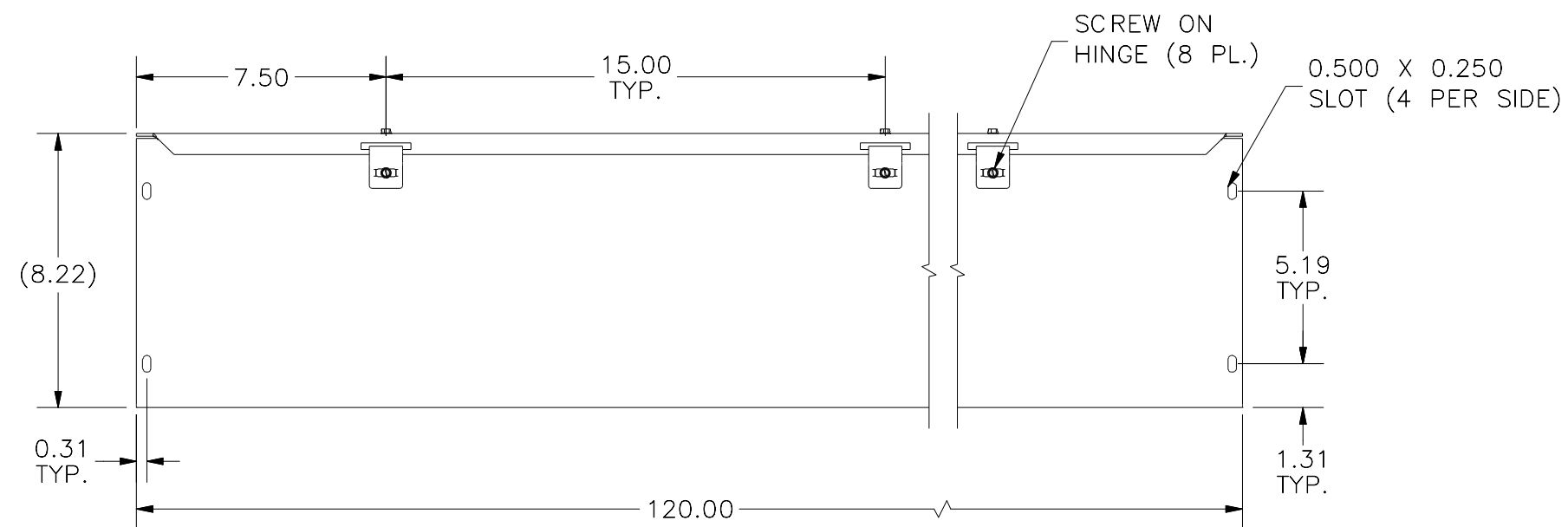
FRONT VIEW
