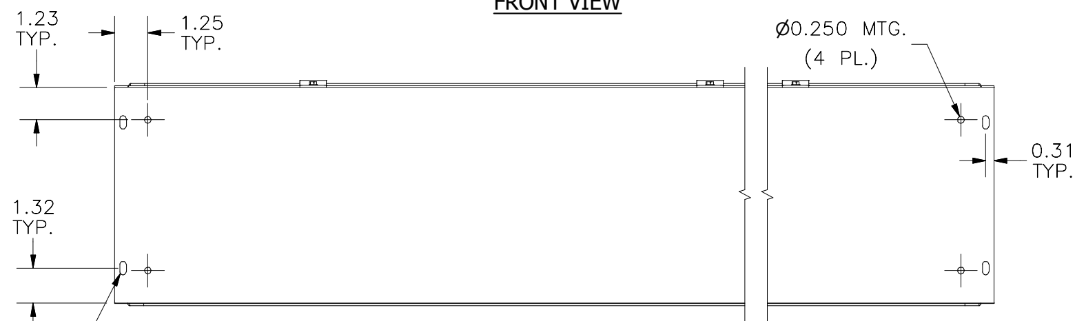
BOTTOM VIEW
