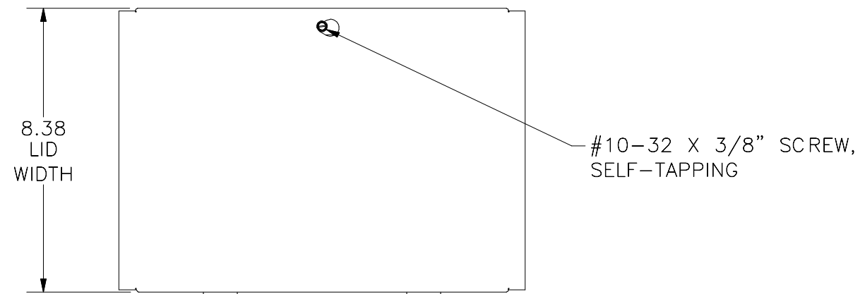
TOP VIEW
