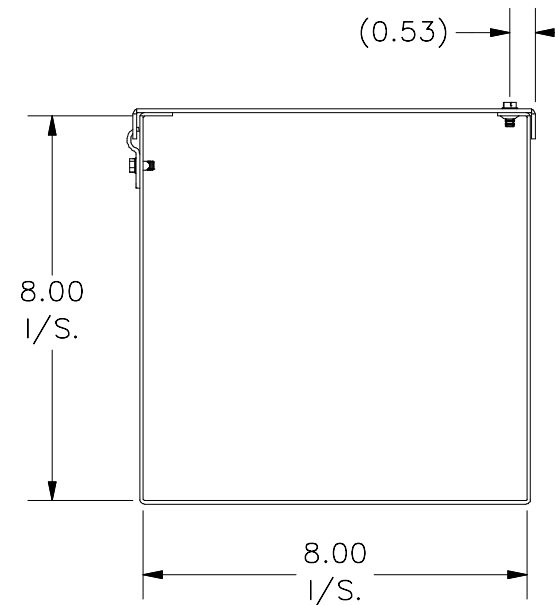
RIGHT VIEW
