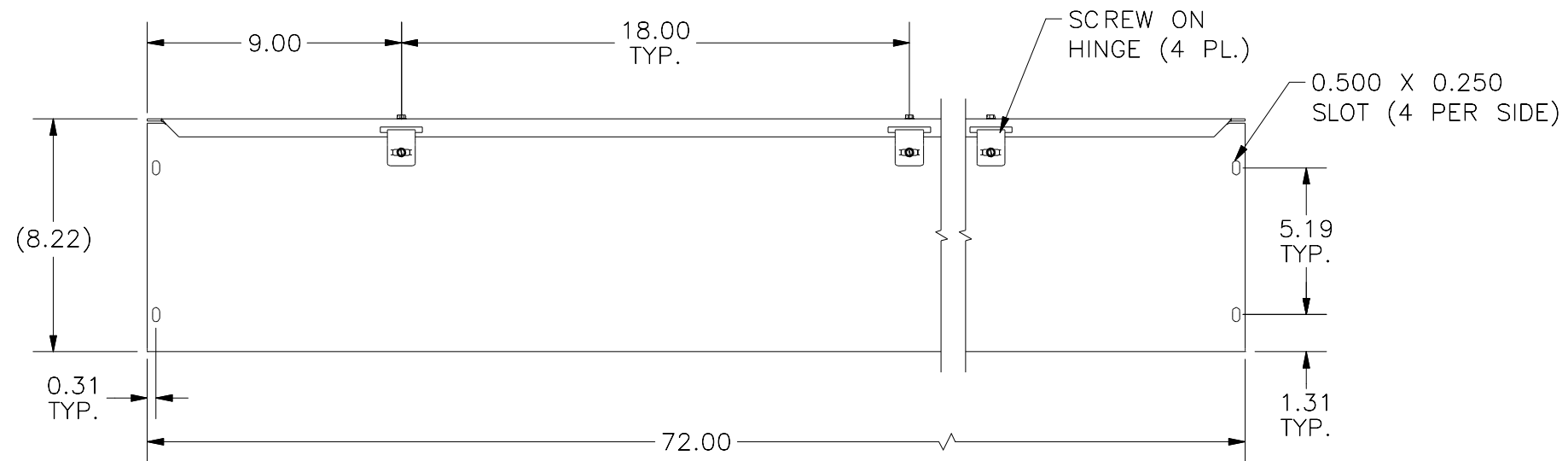
FRONT VIEW
