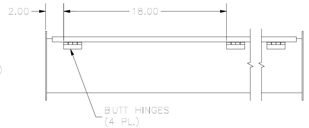
BACK VIEW
