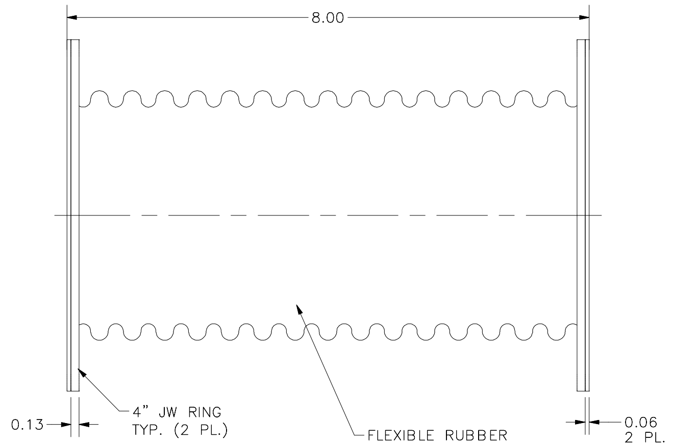
SIDE VIEW
