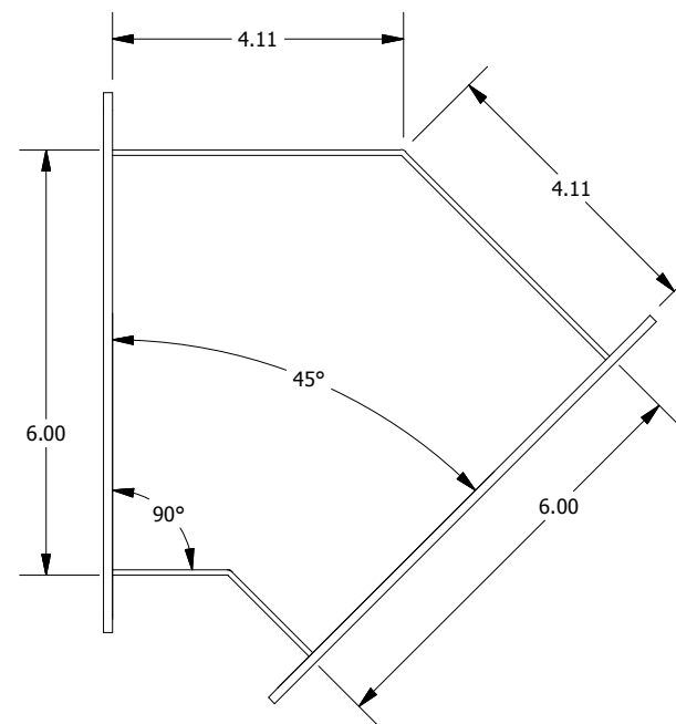
TOP VIEW
