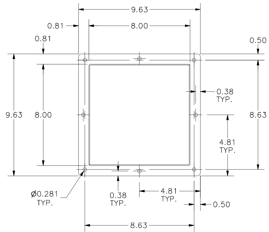
FRONT VIEW
