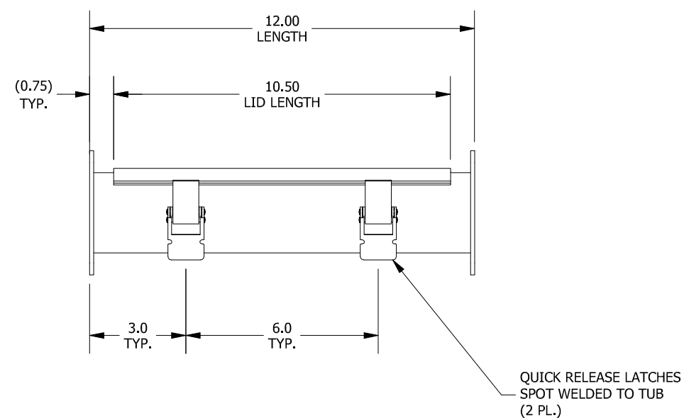
FRONT VIEW
