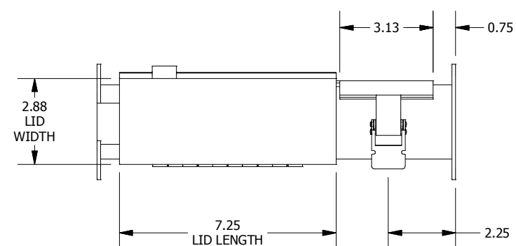
BOTTOM VIEW
