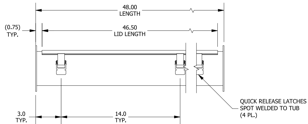
FRONT VIEW
