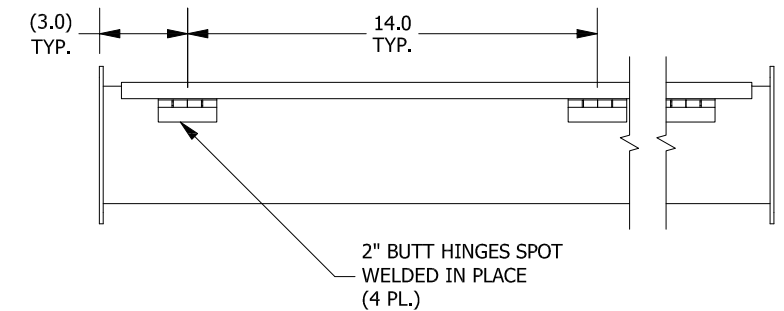
BACK VIEW
