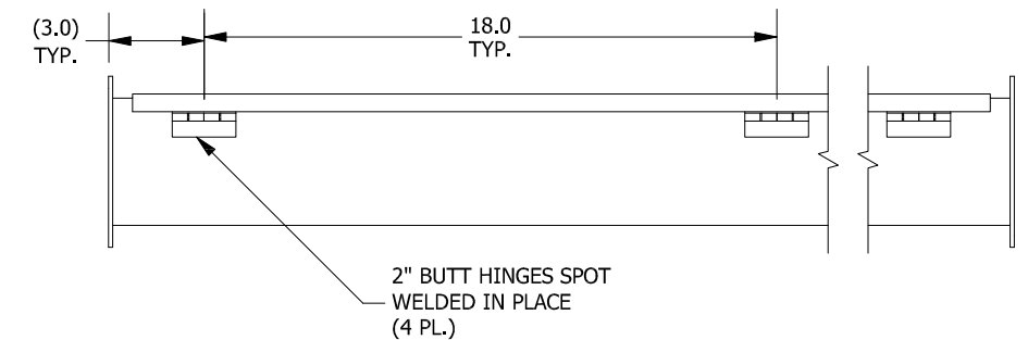
BACK VIEW
