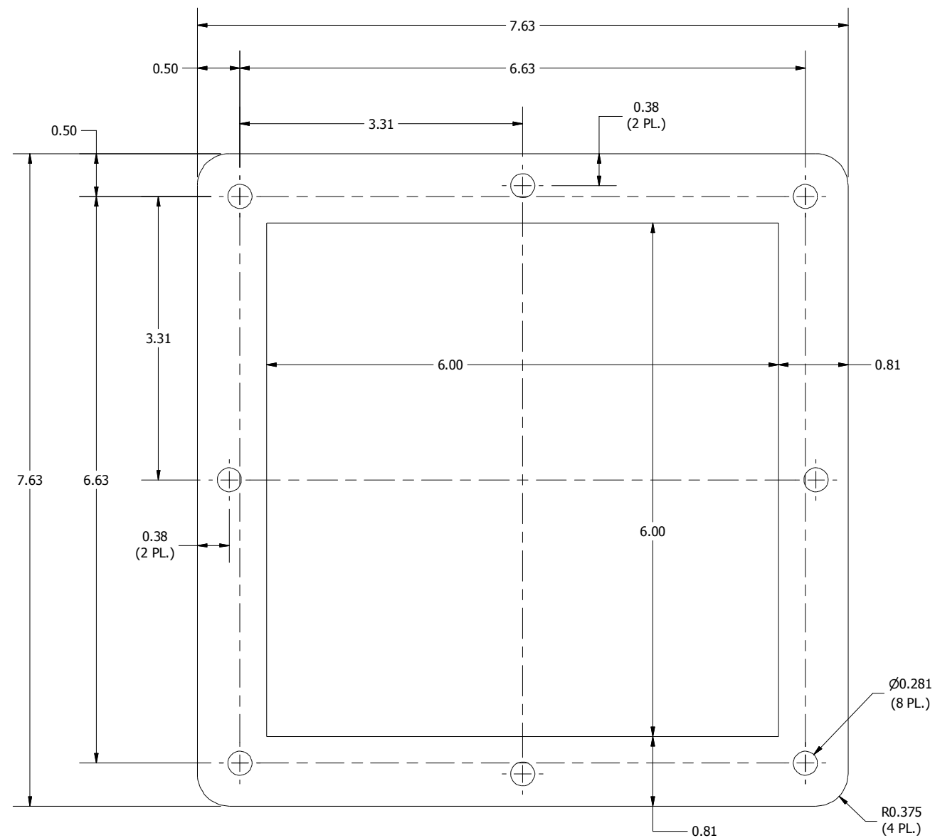
FRONT VIEW
