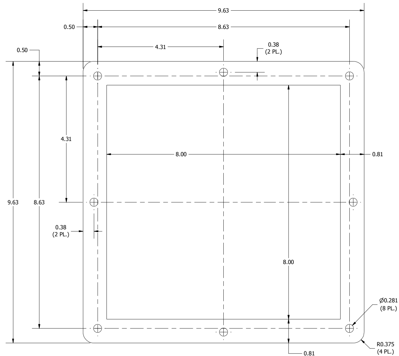
FRONT VIEW
