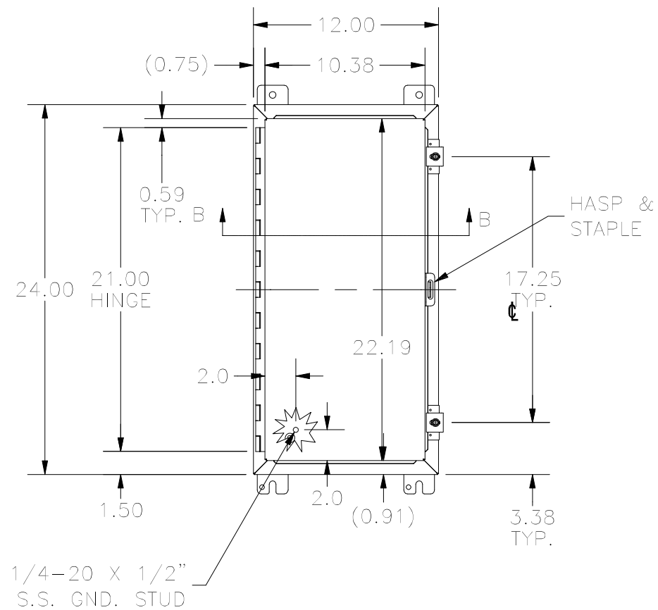
FRONT VIEW
