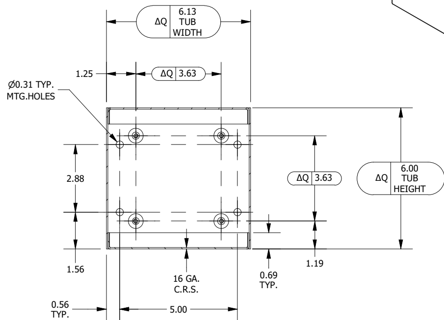
SECTION A-A VIEW (INSIDE BACK OF ENCL.)
