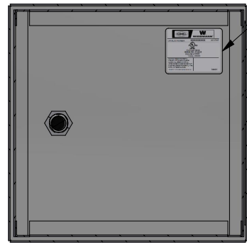
SECTION L-L (CERTIFICATION LABEL VIEW FOR REF.) (FOR LABEL DETAILS, SEE HWDN1C_SMALL_LABELS)
