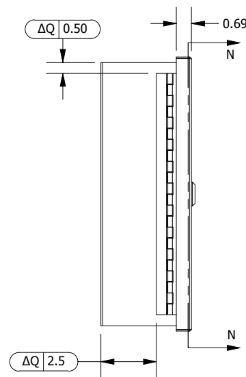
SECTION N-N (CERTIFICATION LABEL VIEW FOR REF.) (FOR LABEL DETAILS, SEE HWDN1C_SMALL_LABELS)
