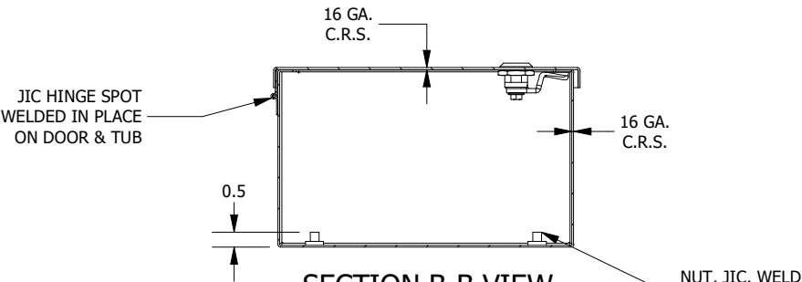
SECTION B-B VIEW (INSIDE TOP OF ENCL.)
