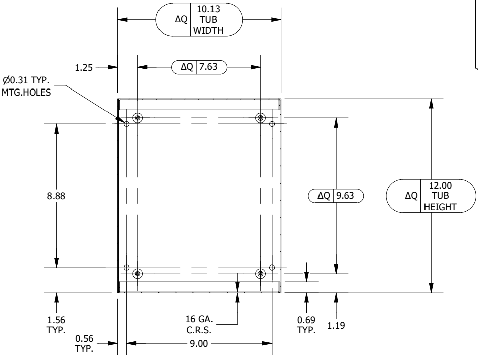
SECTION A-A VIEW (INSIDE BACK OF ENCL.)
