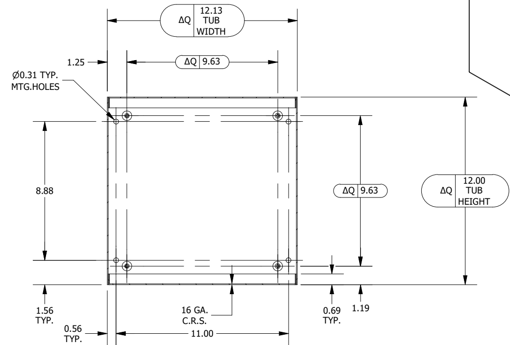
SECTION A-A VIEW (INSIDE BACK OF ENCL.)
