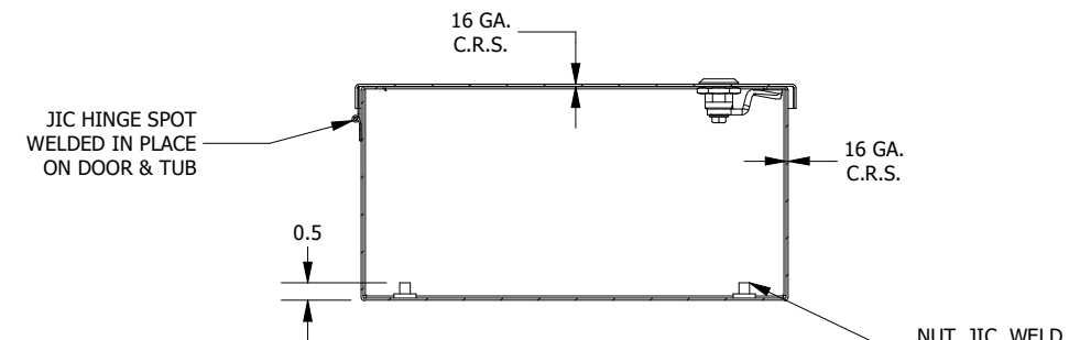
SECTION B-B VIEW (INSIDE TOP OF ENCL.)
